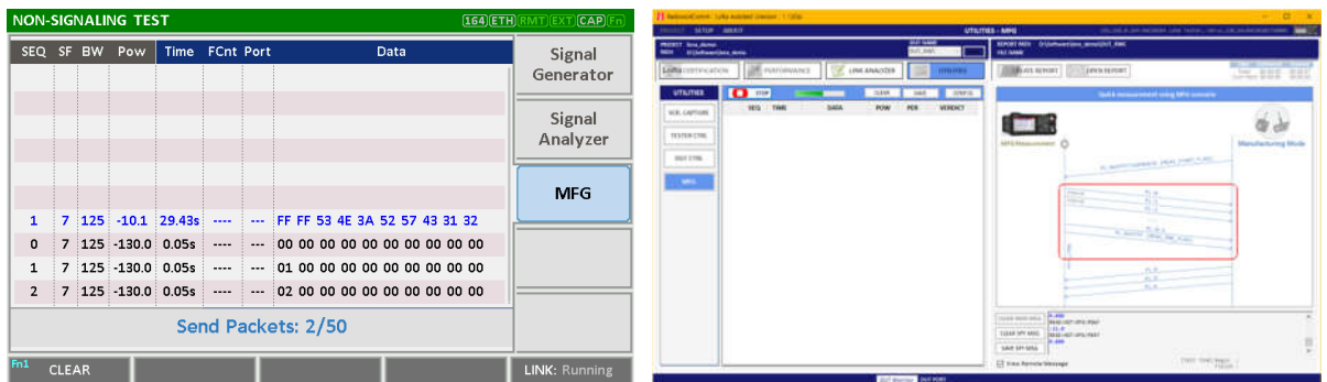
Fig 3.33 The screen of MFG of RWC5020A and PC App. while transmitting packets
