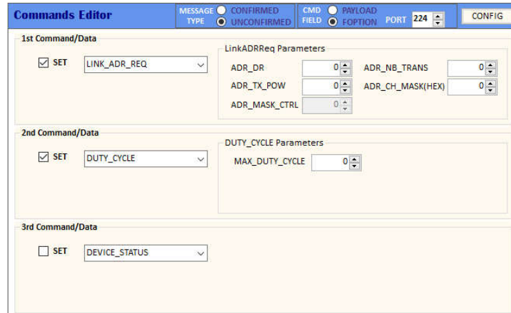
Fig 3.20 Commands Editor
