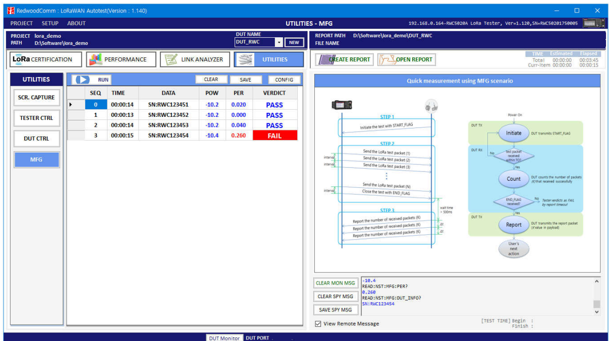
Fig 3.35 Example test using 4 DUTs(N=50, Target PER=0.1)
