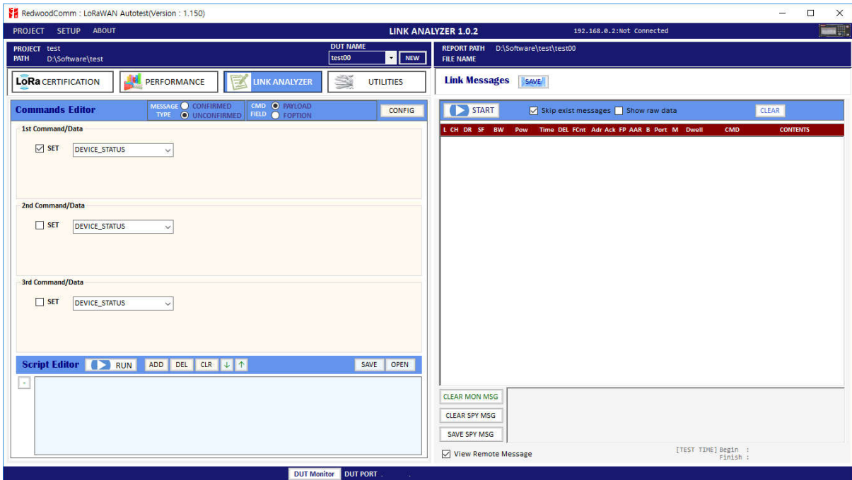
Fig 3.19 Link Analyzer
