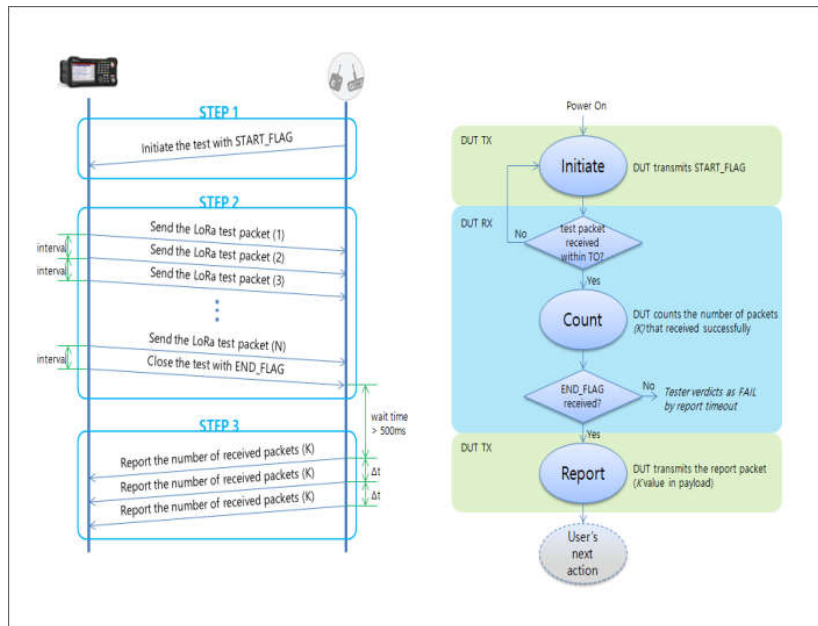
Fig 3.30 Test scenario for manufacturing
