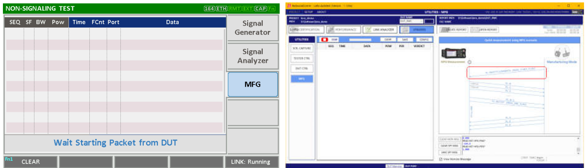
Fig 3.32 The screen of MFGA of RWC5020A and PC App. waiting for MEAS_START_FLAG from DUT
