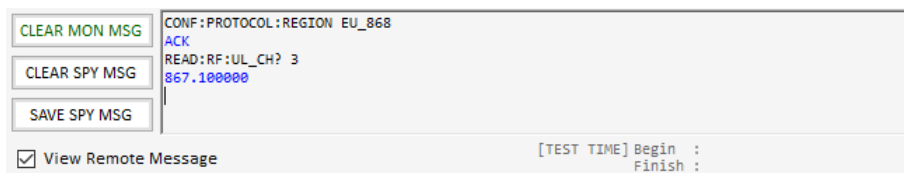
Fig 3.18 Remote Message
