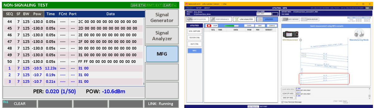
Fig 3.34 The screen of MFG of RWC5020A and PC App. waiting for report frames from DUT
